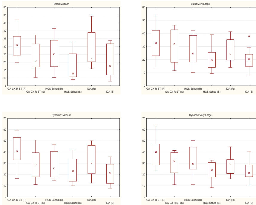
Fig. 4.7: The box-plot of the results for Fail_r parameter in static and dynamic scenarios
