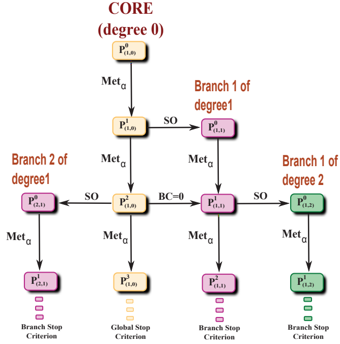
Fig. 4.4: 3 levels of HGS-Sched tree structure
