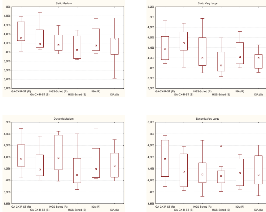
Fig. 4.5: The box-plot of the results for Makespan in static and dynamic scenarios
