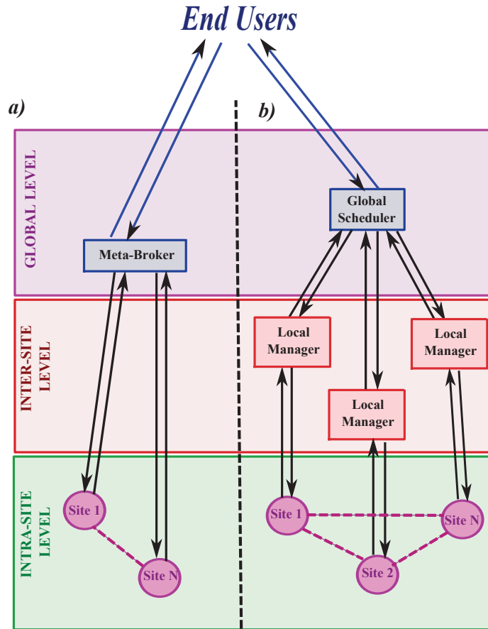
Fig. 4.1: Two-level (a) and three-level (b) hierarchical architecture of clusters in Computational Grids
