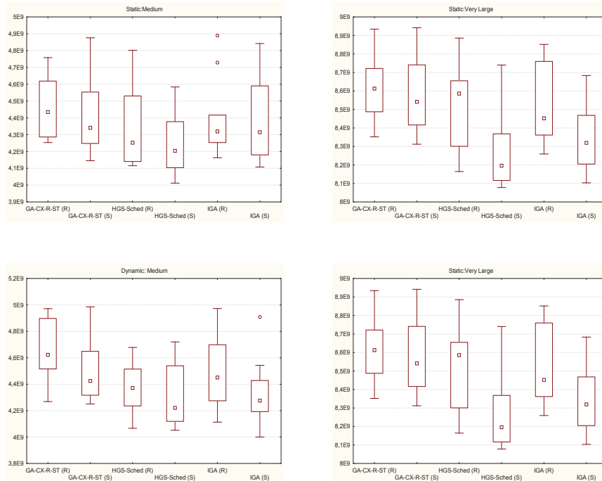
Fig. 4.6: The box-plot of the results for Mean.Flowtime in static and dynamic scenarios
