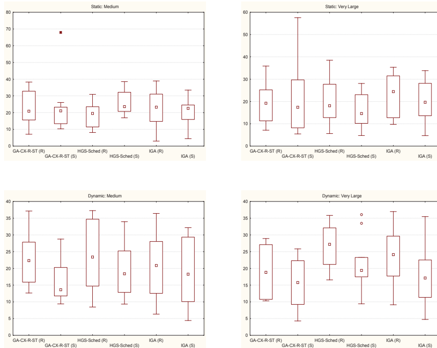
Fig. 4.8: The box-plot of the results for Energy Improvement Rate in static and dynamic scenarios
