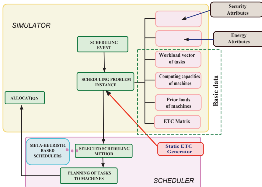
Fig. 4.3: General Flowchart of Security- and Energy-Aware Sim-G-Batch Simulator Linked to Scheduling
